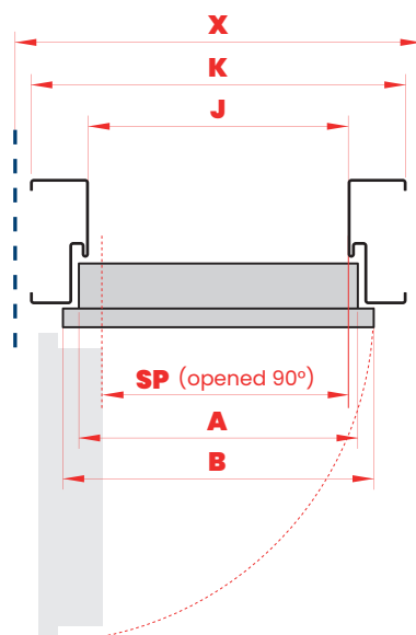
HORIZONTAL CROSS SECTION
