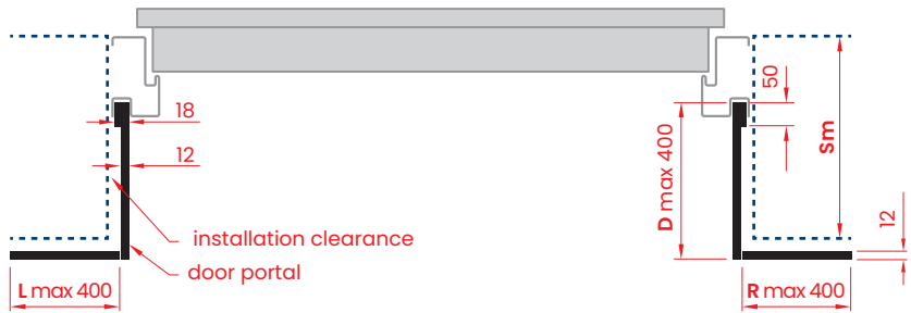
HORIZONTAL CROSS SECTION
