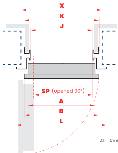
HORIZONTAL CROSS SECTION
