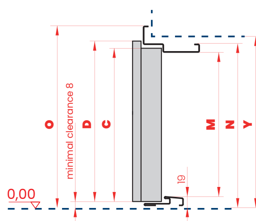
VERTICAL CROSS SECTION
