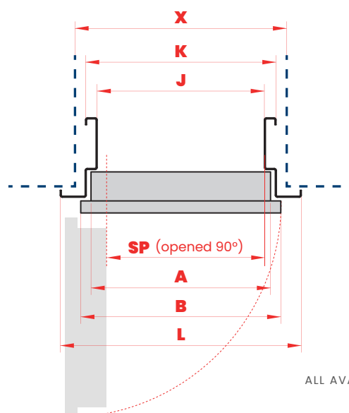
HORIZONTAL CROSS SECTION
