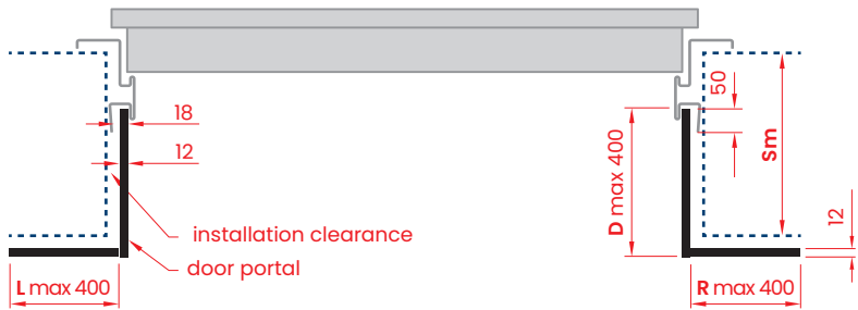
HORIZONTAL CROSS SECTION
