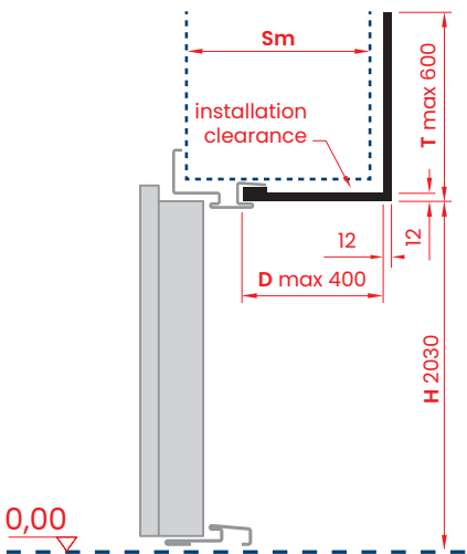
VERTICAL CROSS SECTION
