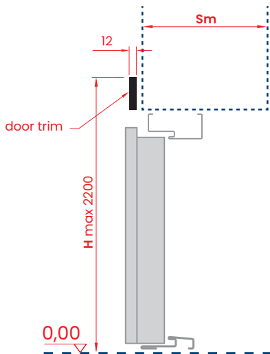
VERTICAL CROSS SECTION
