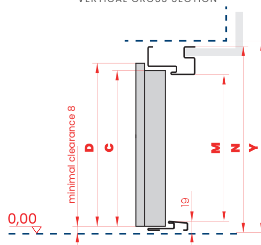
VERTICAL CROSS SECTION
