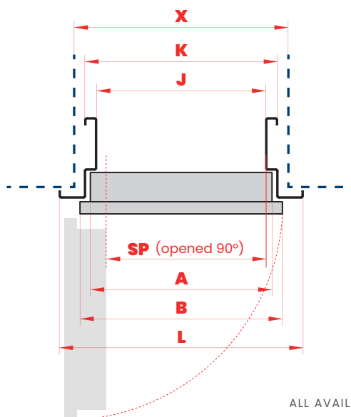
HORIZONTAL CROSS SECTION
